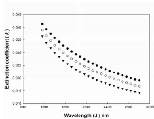
Fig. 3. The variation of extinction coefficient ( k ) against wavelength ( \lambda ) nm, for Pb:GeSbTe chalcogenide thin films.
